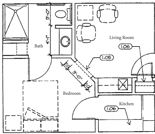
One Bedroom Floor Plan 365 Total Sq. Ft.
