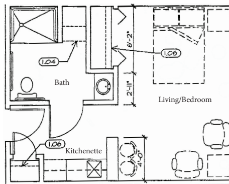
Studio Floor Plan 338 Total Sq. Ft.
