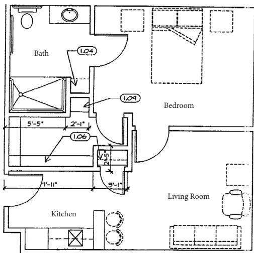
One Bedroom Floor Plan 500 Total Sq. Ft.
